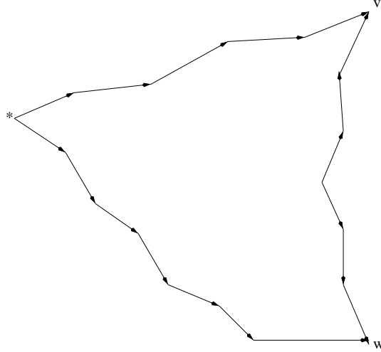
A geodesic triangle in X(\mathcal{G})
