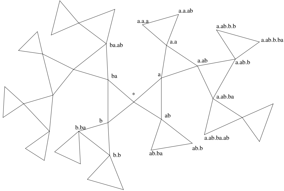
X(\mathcal{G}) for \mathcal{G} = \mathcal{A}/\Delta^2 , \mathcal{A} = \langle a, b \mid aba = bab \rangle
